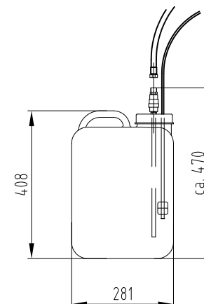
Drinkwater tank 16L
